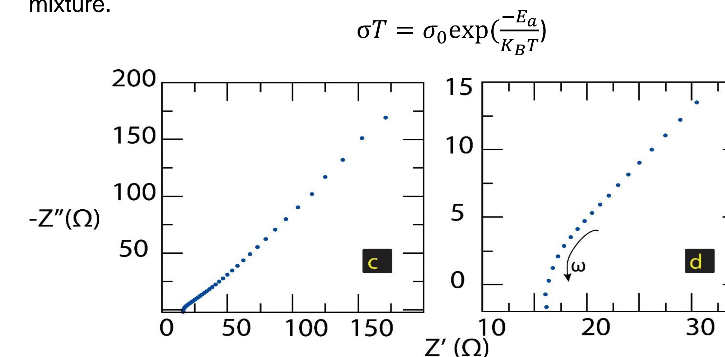
Electrochemical impedance spectra of the fully converted sample (c) at 290°C over the entire frequency range tested, (d) the high frequency regime at 290°C.
