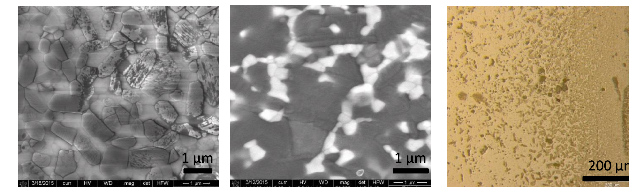
An SEM micrograph of Fe-doped α-Al 2 O 3 + TZ-3Y, (b) An SEM image of the sample after conversion to Fe-doped Na-β"-alumina + TZ-3Y (c) An optical micrograph showing the boundary between the converted and the unconverted sample.
