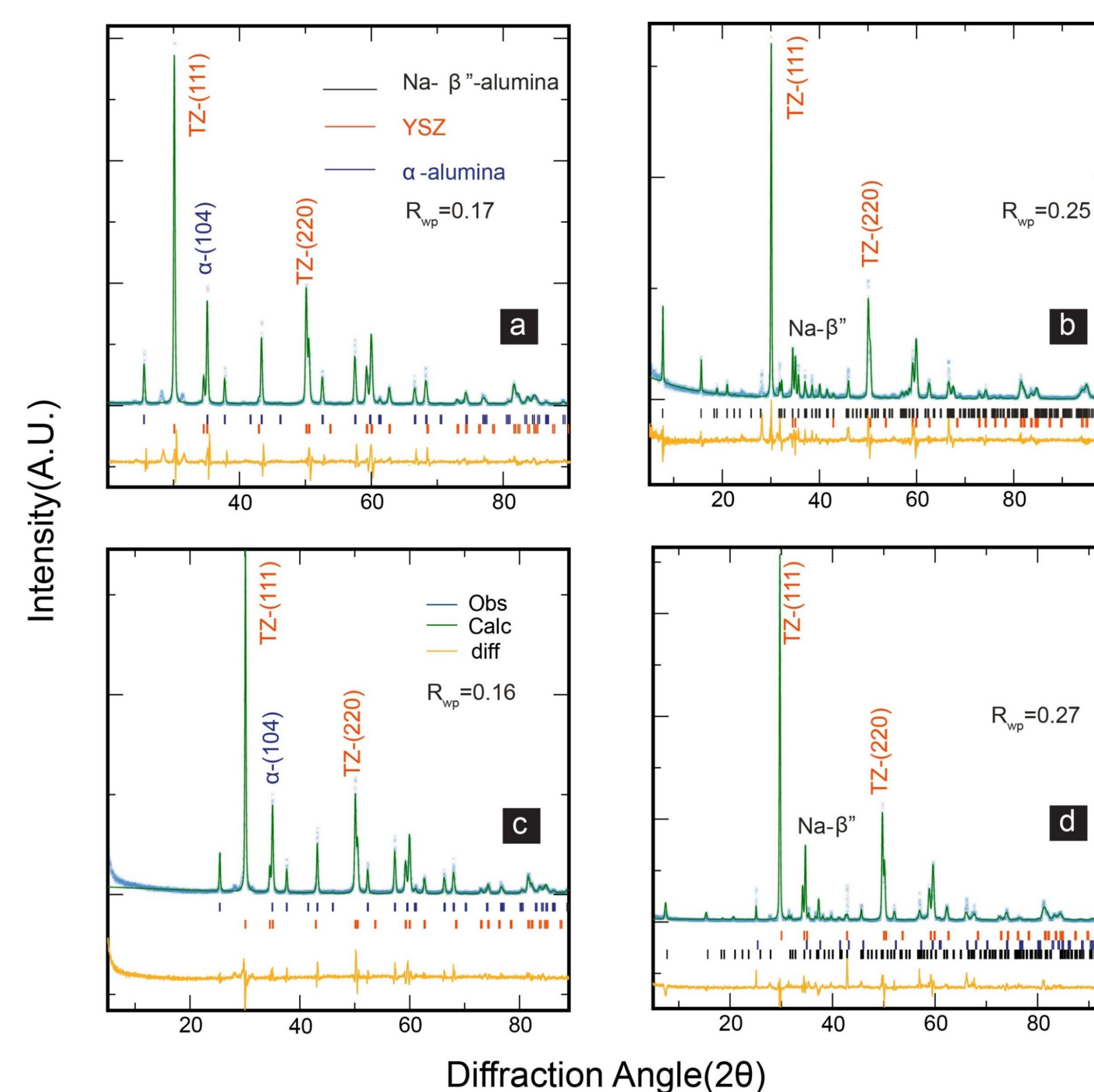
Refined histograms of α-Alumina/YSZ, b- Na-β"-alumina/YSZ, c- iron doped Alumina/YSZ before conversion and d- iron doped Alumina/YSZ after conversion Comparison of lattice parameters determined by refinement and Vegard's Law indicate that hematite is completely dissolved in the alumina structure.
