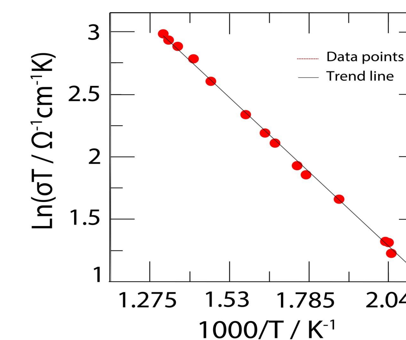
Arrhenius plot of the fully converted sample.
